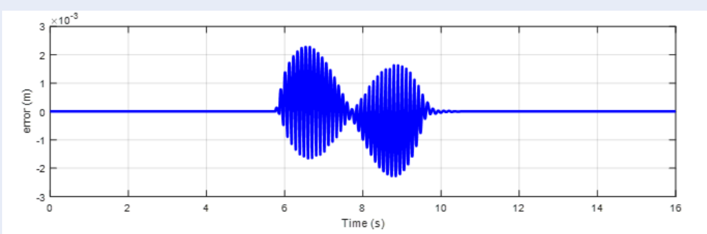
Figure 9: The deviation between planned path and actual path.
