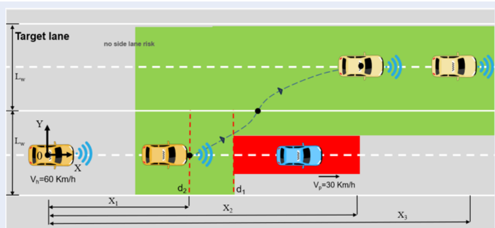
Figure 4: The host car's navigation zone delimited by the green zone and generated reference trajectory zones.
