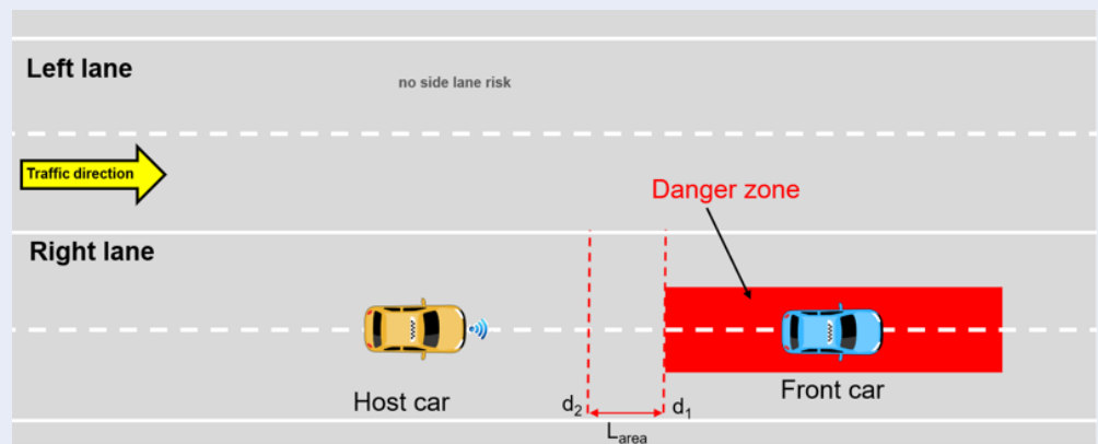
Figure 3: The danger zones of front car for the host car with L_{area} is the length of the lane changing area
