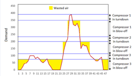
Figure 3: Wasted air when applying start/stop control and load/unload control.
