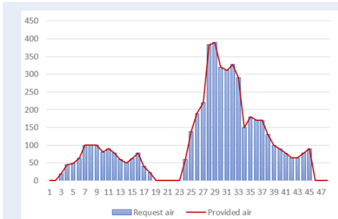
Figure 11: The operating schedule with 4 compressors can satisfy the demand.
