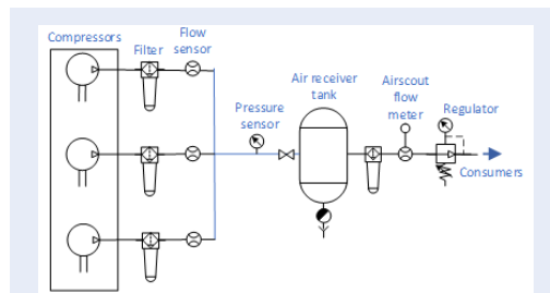
Figure 1: A compressed air network system.
