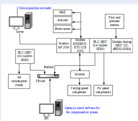
Figure 5: PLC control system for the testbed.
