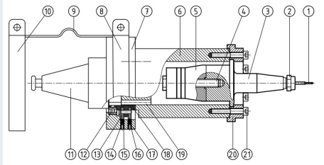
Figure 2: Ultrasonic vibration-assisted machining tool (UVAM) 15
