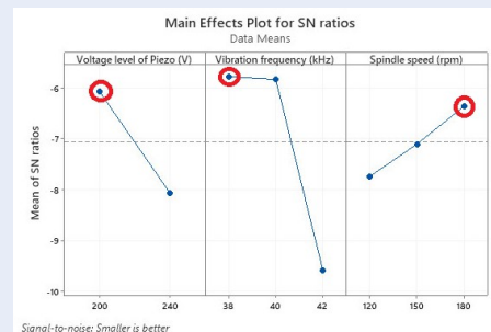
Figure 7: The graph shows the influence of technological parameters according to the survey values on the surface roughness index Ra.
